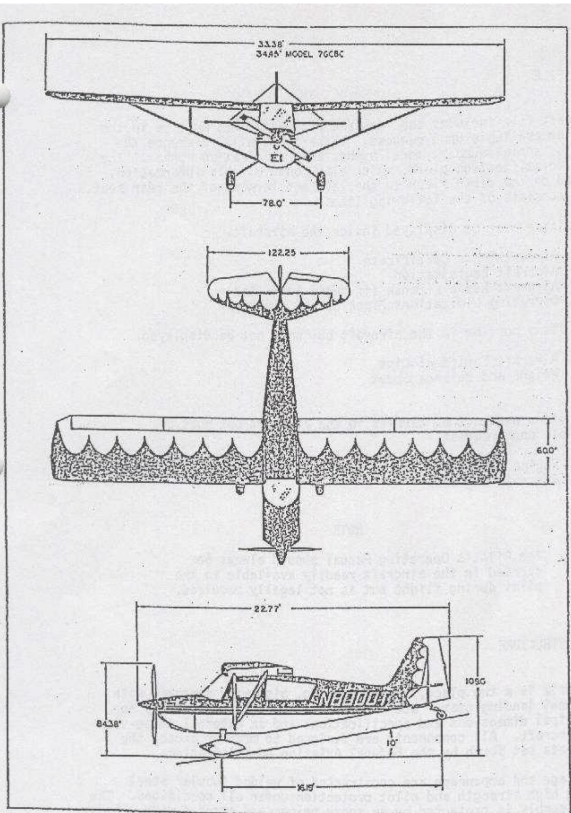
FIGURE 6-2 CITABRIA THREE-VIEW
